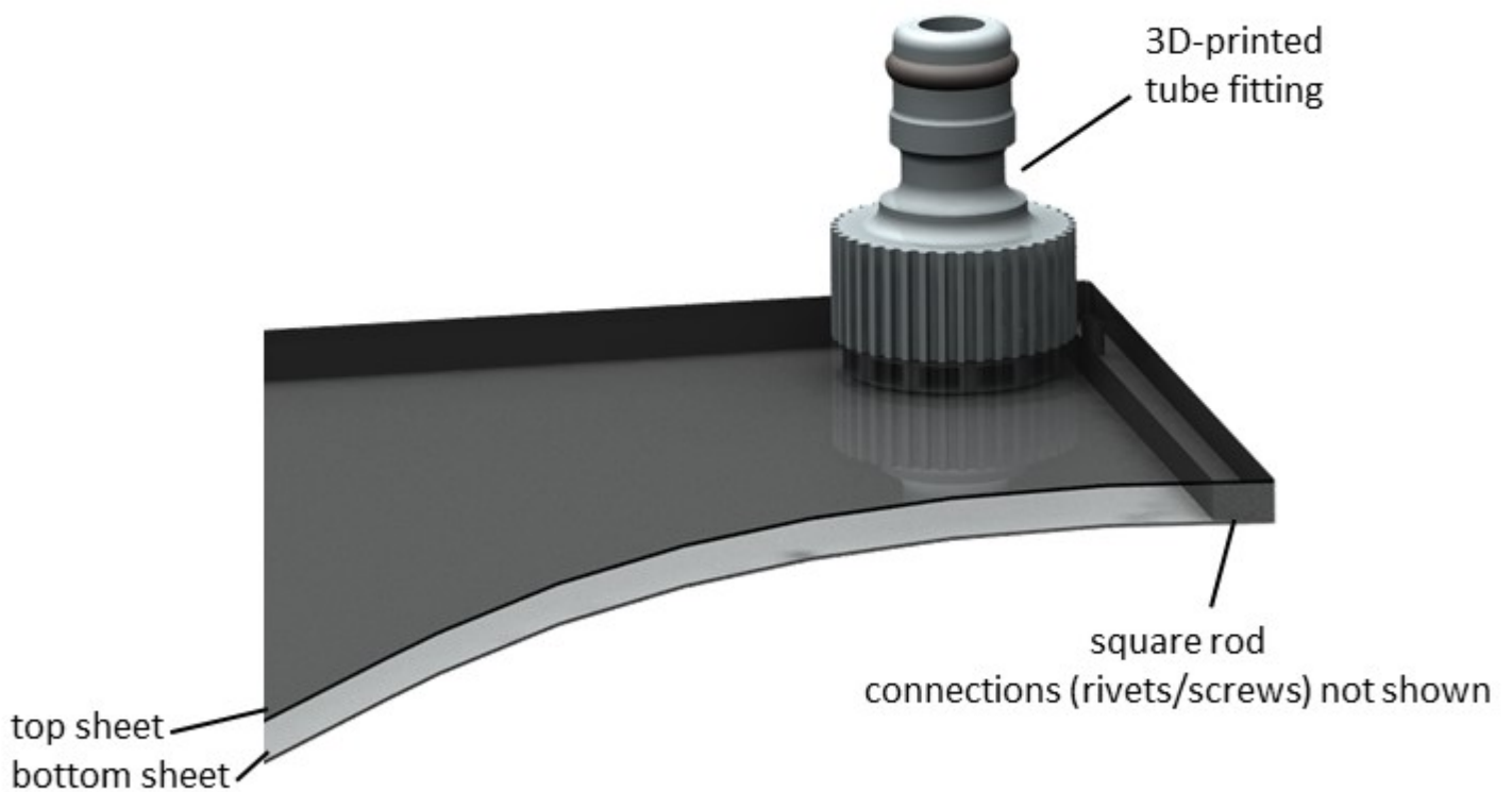
Broken-out view (top sheet rendered as glass to show inside)
